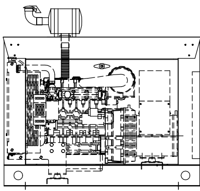
DRAWING DEPICTS UNIT WITH OPTIONAL EQUIPMENT
